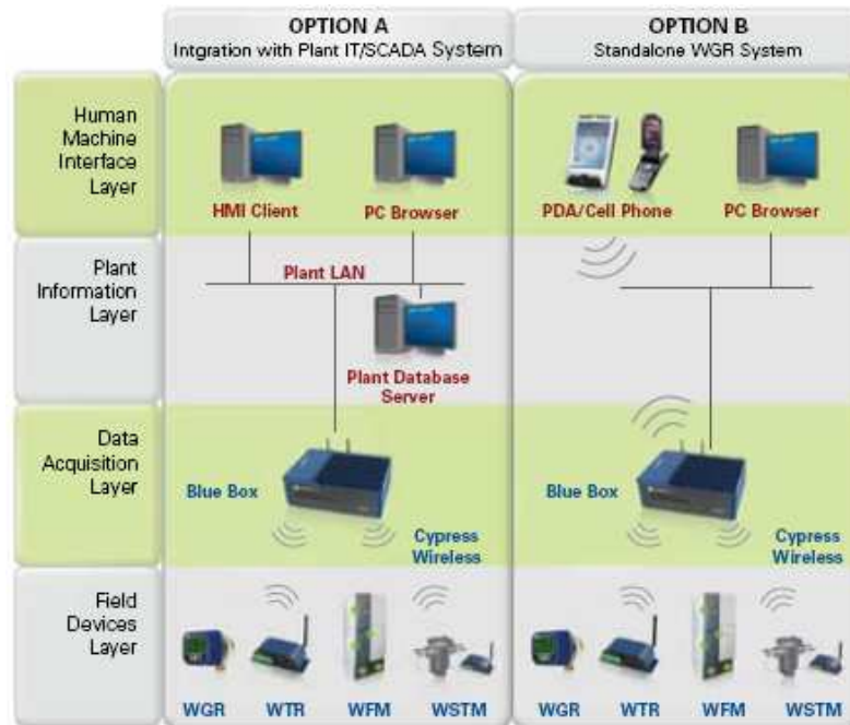
Figure 3. Cypress Envirosystems Monitoring System Setup Options
