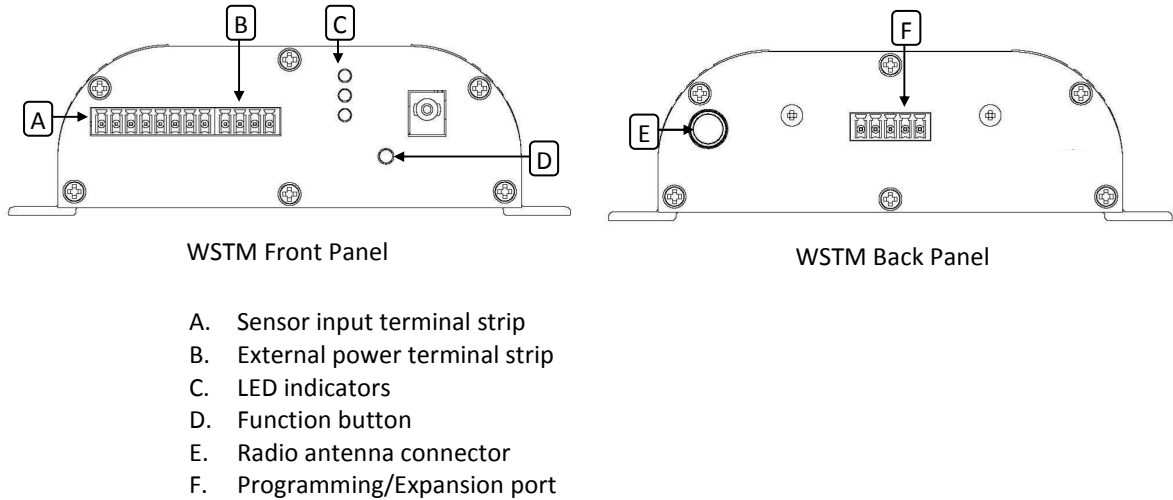
Figure 2. WSTM Schematic
