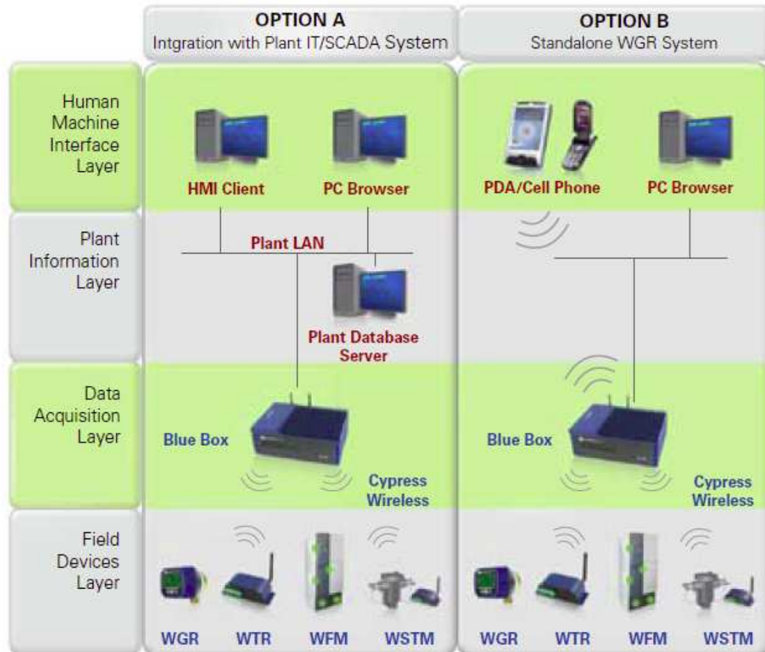
Figure 4. Cypress Envirosystems Monitoring System Setup Options
