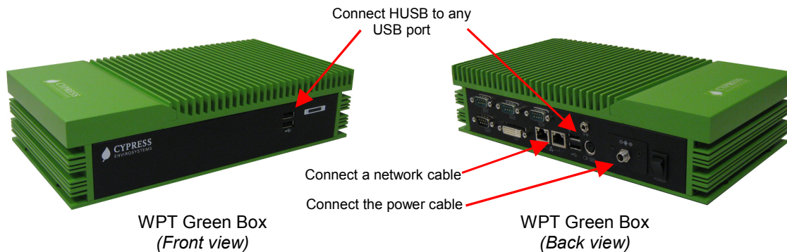
Figure 1. Connections to the WPT Green Box
