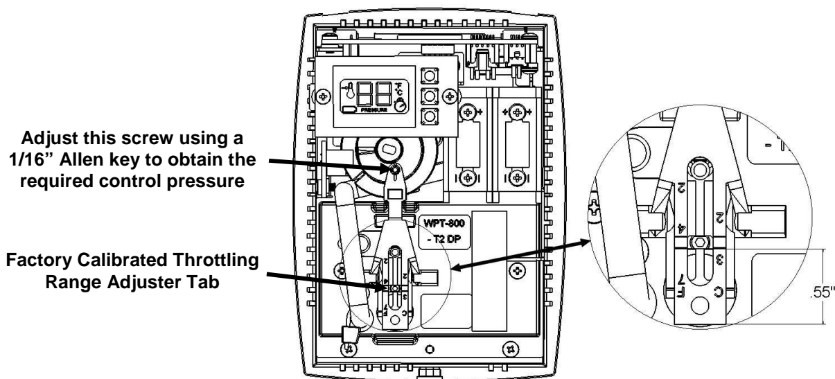
Figure 14. WPT-DB Calibration
